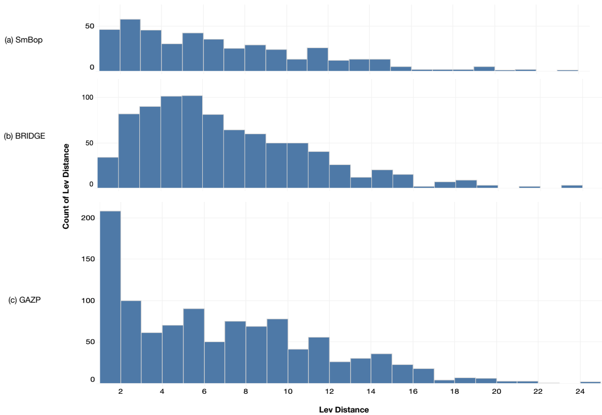
Figure 3: The distribution of Levenshtein distances between erroneous queries and ground truth queries among three models
